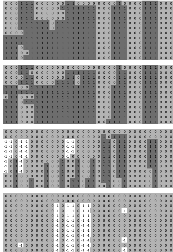
Figure 2. From top to bottom, fingerprints of crises B, B, C and D from Table 1. Each row is an epoch and each column represents the state of a particular metric quantile, with white, gray, black corresponding to cold, normal, hot ( -1, 0, +1 ) respectively in the fingerprint. The fingerprints are composed of 11 metrics, where each three adjacent columns represent three quantiles (25 th , 50 th , and 95 th ). Notice that the patterns of metric quantiles in crises B are very similar, while very different from crises C and D.
